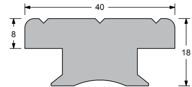
size 40x8 mm fasteners: Ø8 mm screws any length up to 6 m page 100
