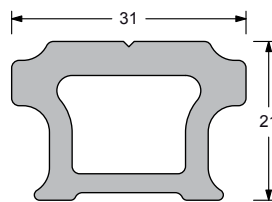
size 31x21 mm fasteners: Ø8 mm screws any length up to 6 m page 116
