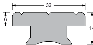
size 32x6 mm fasteners: Ø6 mm screws any length up to 6 m page 98
