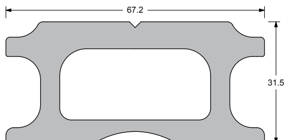
size 67x31.5 mm fasteners: Ø12 mm screws any length up to 6 m page 132
