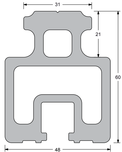
size 31x60 mm fasteners: Ø8 mm screws on sliding slugs any length up to 6 m page 116
