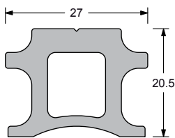
size 27x20 mm fasteners: Ø6 mm screws any length up to 6 m page 113
