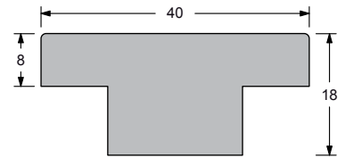
size 40x8 mm fasteners: Ø8 mm screws any length up to 6 m page 108
