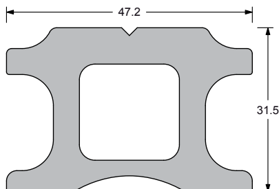
size 47x31.5 mm fasteners: Ø10 mm screws any length up to 6 m page 128
